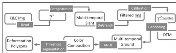
Figure 5. Methodological procedure proposed to classify deforestation based on PALSAR ScanSAR multi-temporal series
