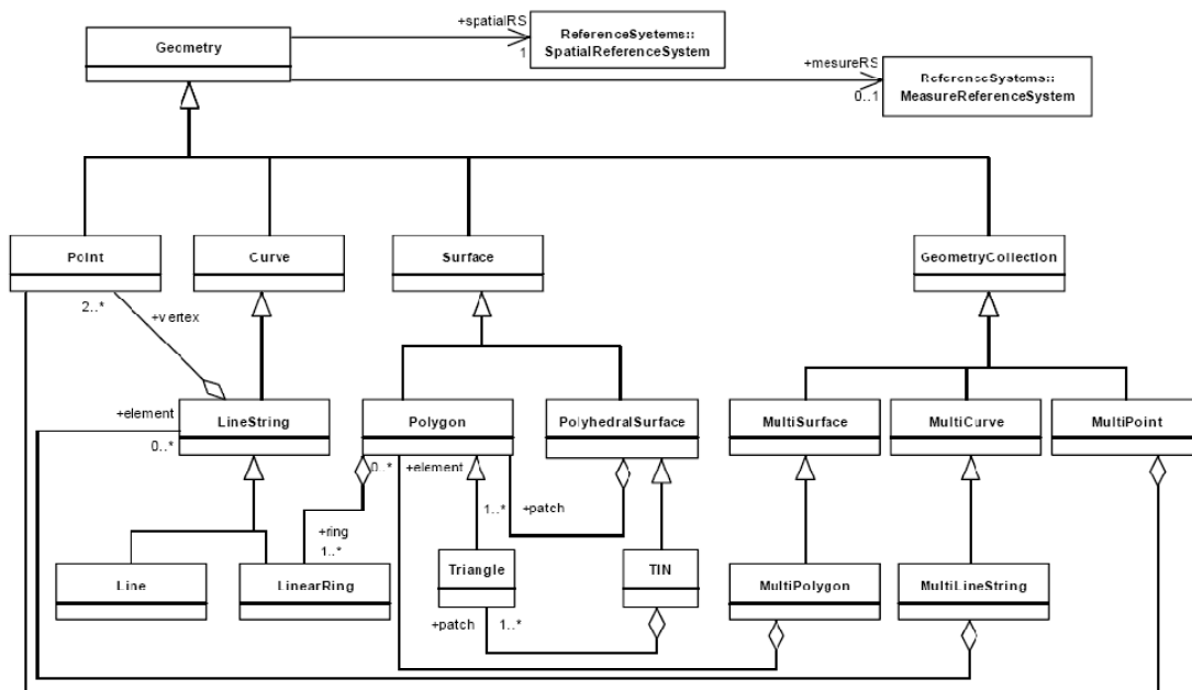
Figure 2.5 – Geometry class hierarchy
