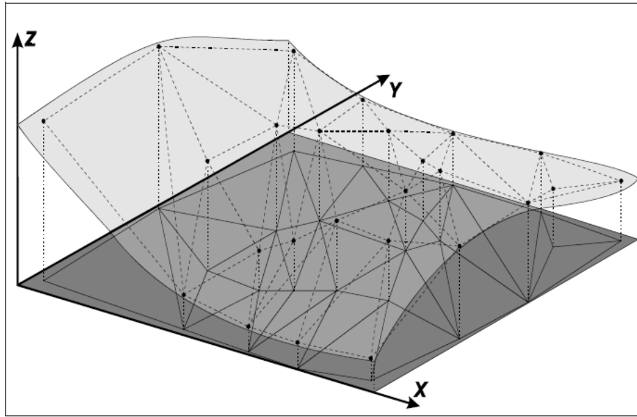
Figure 2.2 – Example of irregular grid
