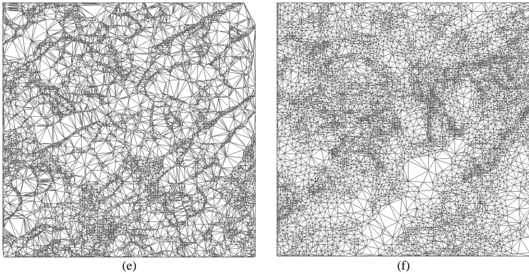
Figure 4.2 – Comparison of Multiscale TIN from Mount Marcy dataset with 80% (a) our method (b) MT, 50% (c) our method (d) MT, and 20% (e) our method (f) MT.
