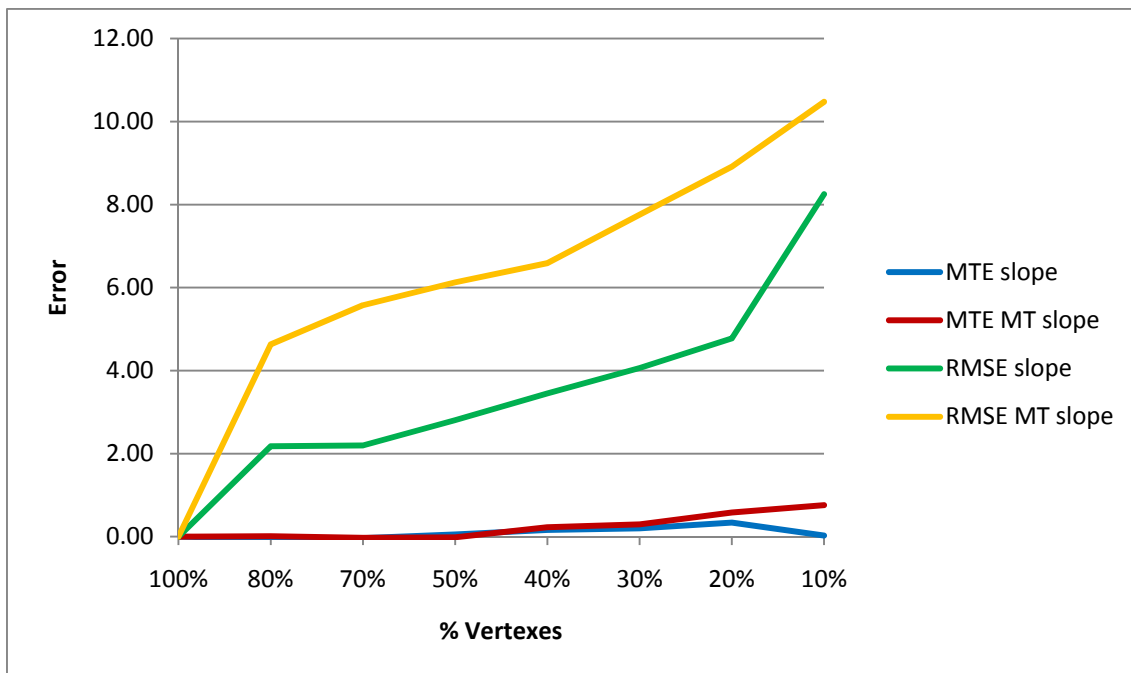
Figure 4.4 – MTE and RMSE slope values for TIN from Mount Marcy with different number of vertexes.
