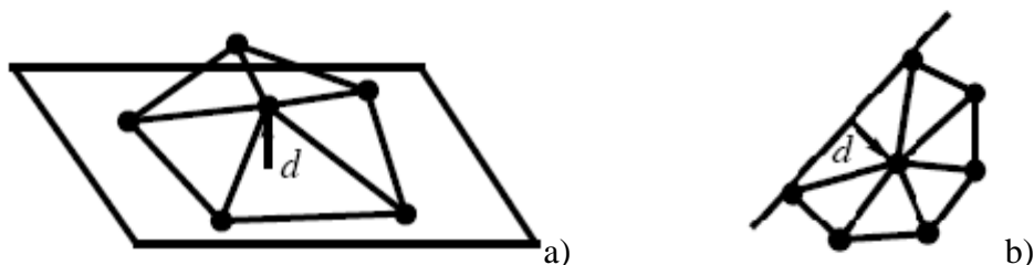
Figure 2.3 – Decimation criterion a) average plane b) edge criterion
