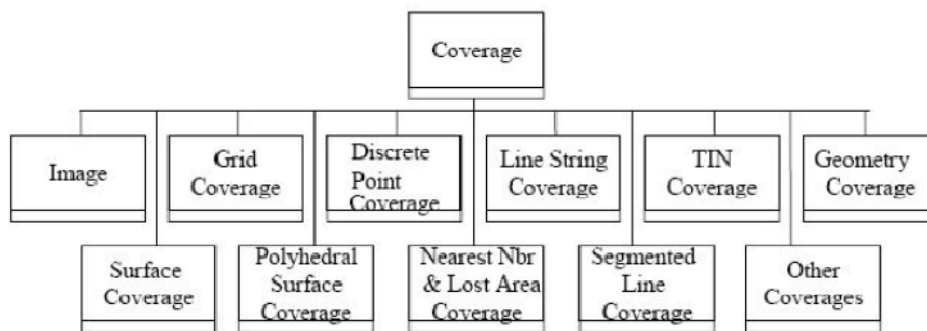
Figure 2.7 – Coverage subtypes
