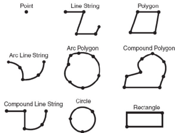
Figure 2.12 – Geometric types from Oracle Spatial Source: Murray (2009)
