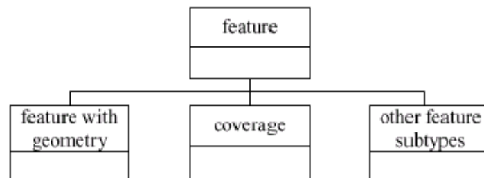
Figure 2.4 – Feature subtypes
