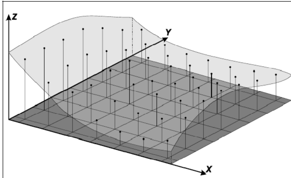
Figure 2.1 – Example of regular grid
