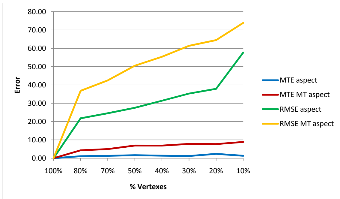
Figure 4.5 – MTE and RMSE aspect values for TIN from Mount Marcy with different number of vertexes.
