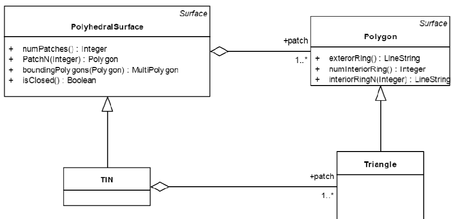
Figure 2.6 – PolyhedralSurface class
