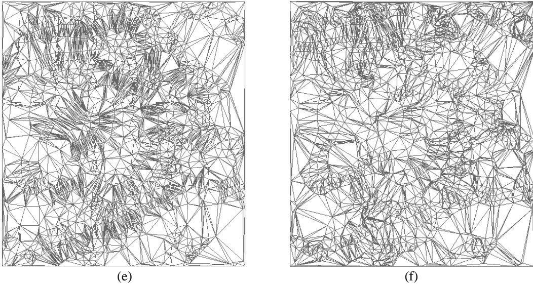
Figure 4.3 – Comparison of Multiscale TIN from Brasilia dataset with 60% (a) our method (b) MT, 40% (c) our method (d) MT, and 20% (e) our method (f) MT.
