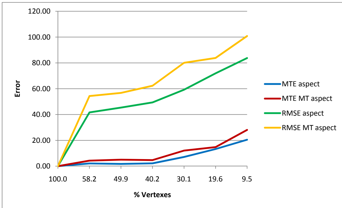
Figure 4.7 – MTE and RMSE aspect values for TIN from Brasilia with different number of vertexes.
