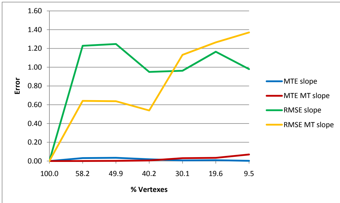
Figure 4.6 – MTE and RMSE slope values for TIN from Brasilia with different number of vertexes.
