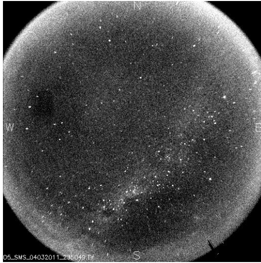
Figure 1 – All-sky image obtained in São Martinho da Serra-RS
