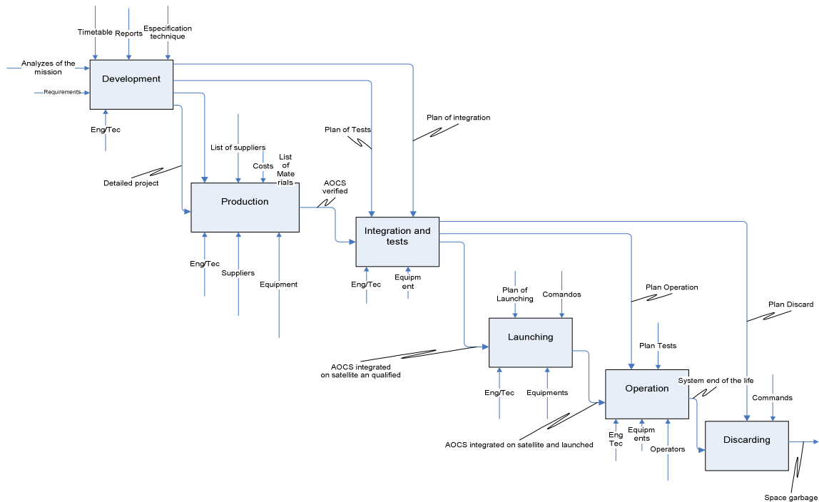
Figure 2. IDEF0 Diagram of the AOCS.
