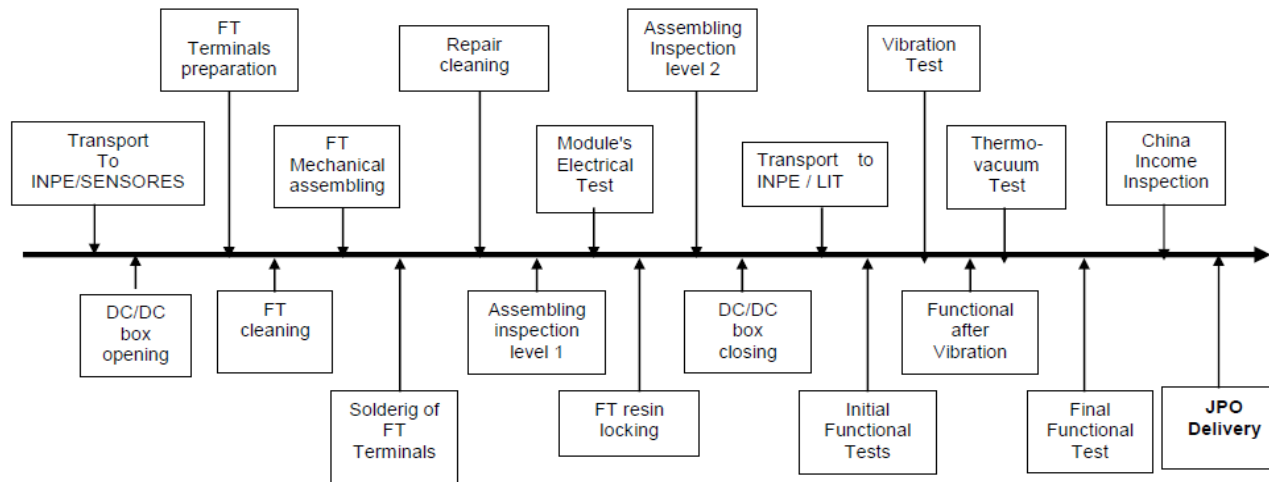
ACTIVITIES FLOWCHART OF DC/DC CONVERTERS REWORK
