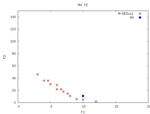
Figure 9: M_4 : Pareto front for t_5
