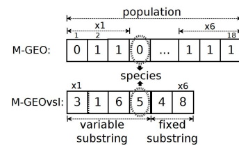
Figure 1: M-GEO × M-GEO vsl : population
