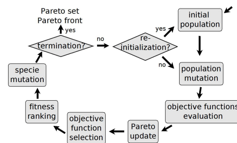
Figure 3: M-GEO vsl : evolution process
