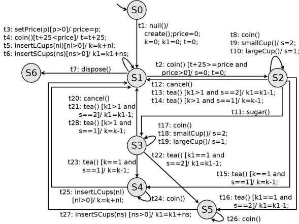
Figure 4: EFSM M_1 for a vending machine
