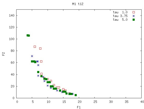
Figure 7: Influence of \tau in M-GEO vsI
