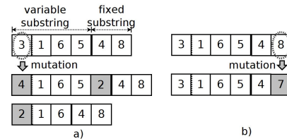
Figure 2: M-GEO vsl : mutations
