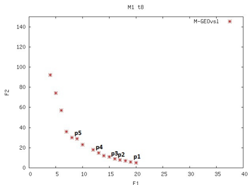
Figure 8: M_1 : Pareto front for t_8
