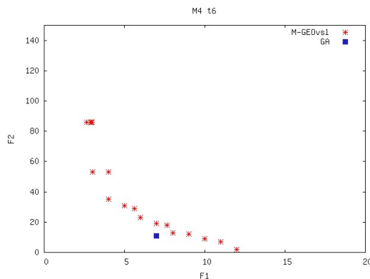
Figure 10: M_4 : Pareto front for t_6
