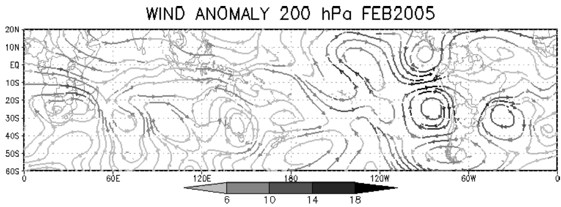
Figure 7. Fields for February 2005 (a) SST anomaly ( ^{\circ}\text{C} ), (b) OLR anomaly ( \text{W}/\text{m}^2 shaded), (c) wind anomaly streamlines at 200 hPa ( \text{m}/\text{s} ).
