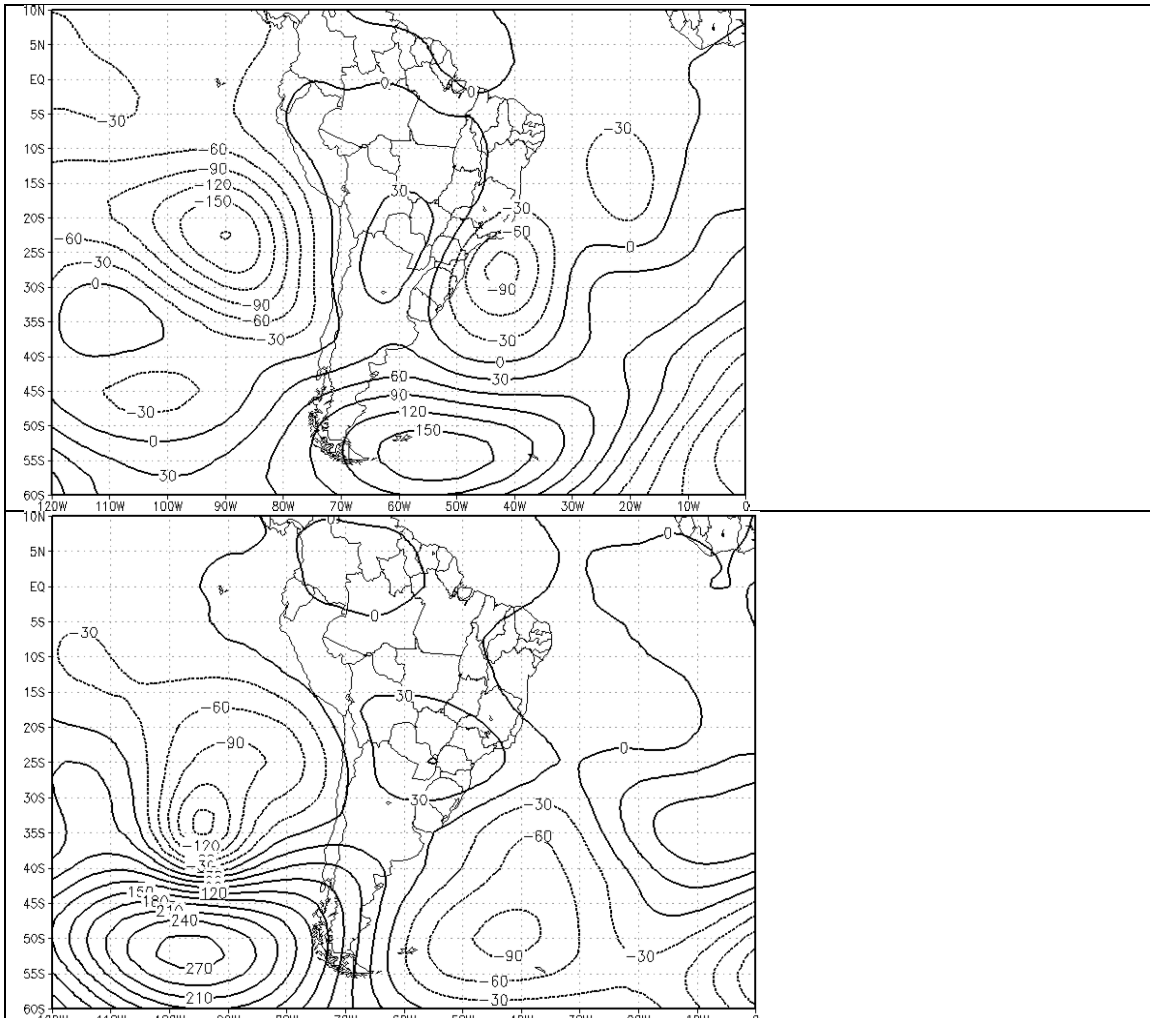
Figure 2. (a) Geopotential anomaly at 200 hPa (mgp) for February 2005. Zonally asymmetric component of geopotential (mgp) at 200 hPa during the two blocking periods (b) 13-22 February 2005, (c) 23-28 February 2005.
