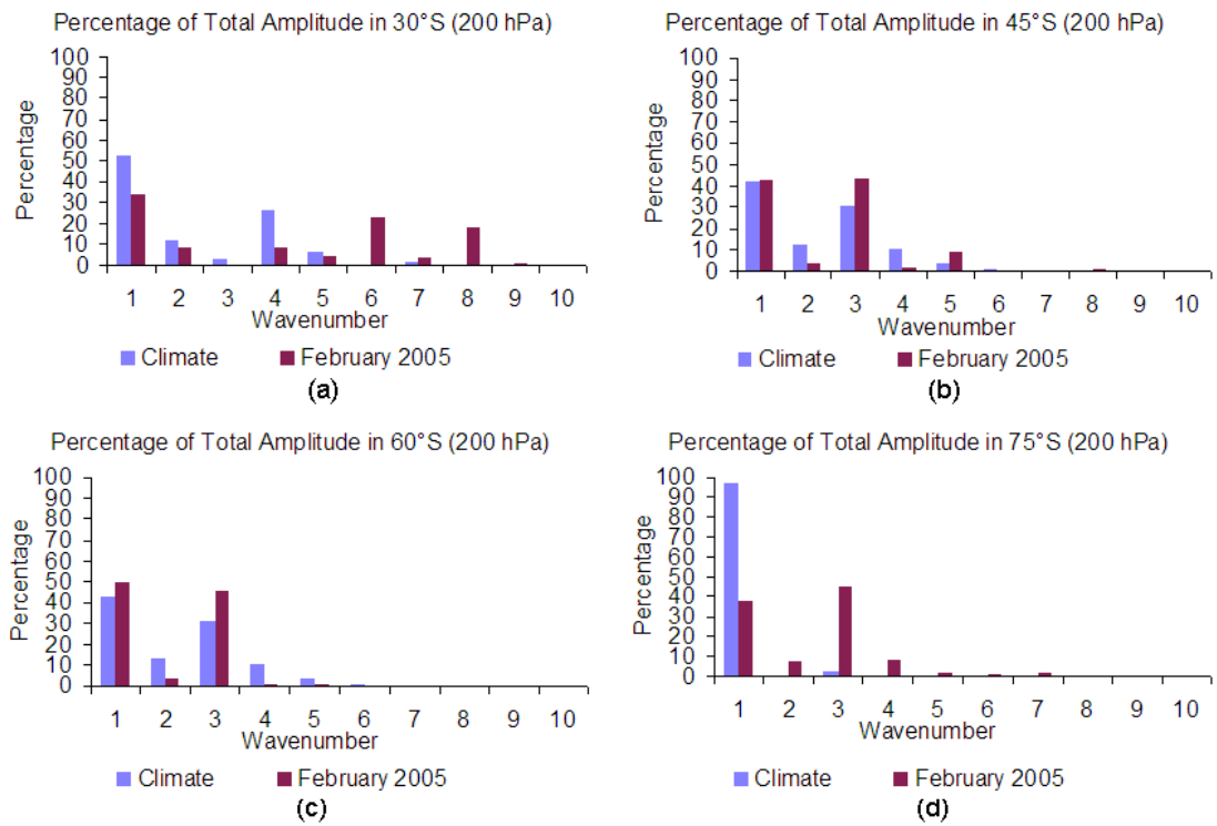
Figure 3. Percentage of geopotential amplitudes at 200 hPa contributed by each wave in February 2005 compared to climatology (a) 30°S, (b) 45°S, (c) 60°S, (d) 75°S.
