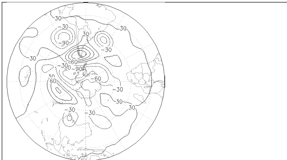
Figure 1. Anomaly fields for February 2005 (a) precipitation anomaly (mm), (b) Sea Level Pressure (hPa), (c) omega at 500 hPa (Pa/s), (d) vertically integrated humidity flux anomaly (kg/m.s), (climatology is taken from 1979 to 2006).
