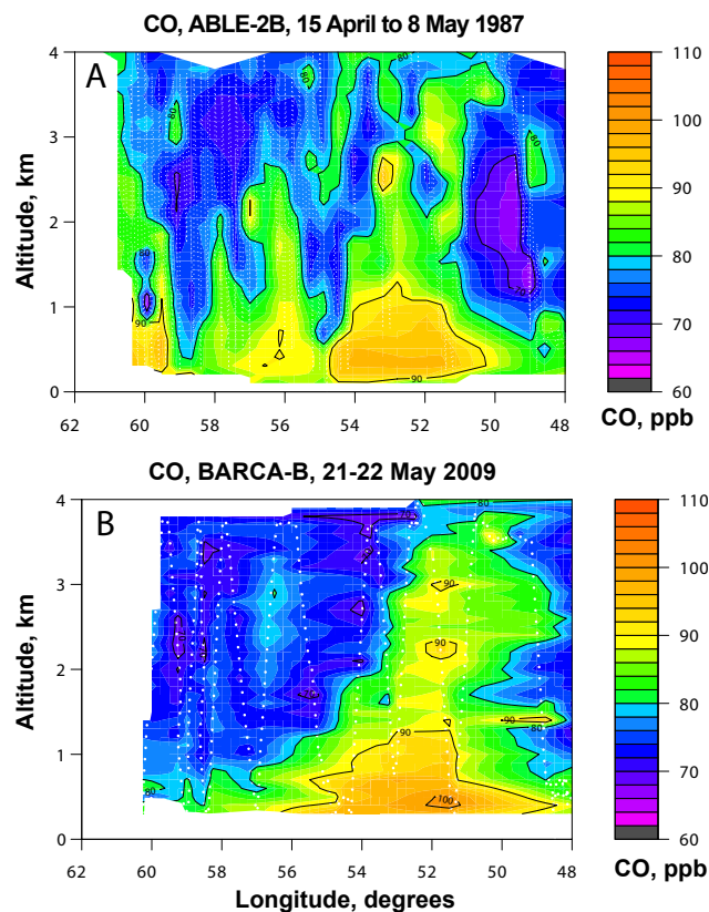
Fig. 9. Cross sections of CO mixing ratios from (A) ABLE-2B (15 April–8 May 1987) and (B) BARCA-B (21–22 May 2009) along the equator ( \pm 4^\circ ). Urban data and a fresh smoke plume were omitted from the data. White dashed lines show flight tracks.
