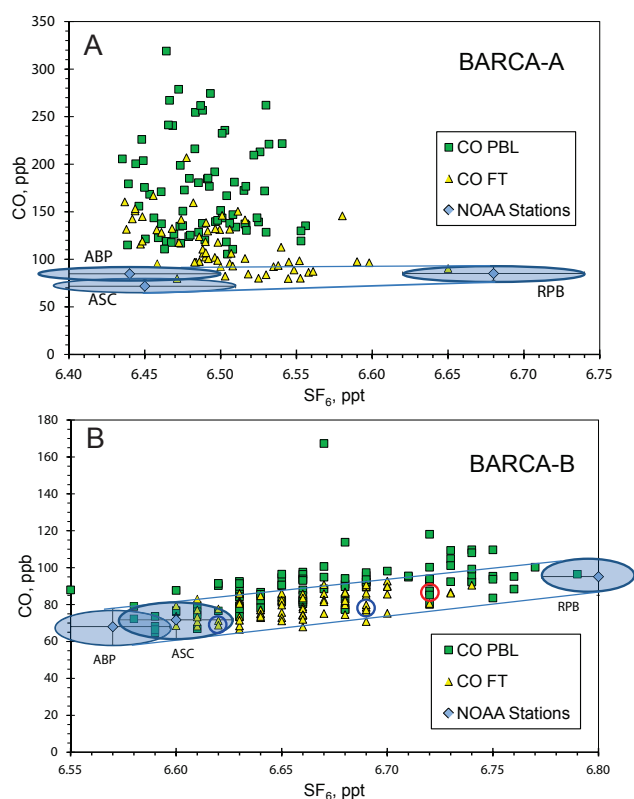
Fig. 4. Plot of CO from the flask samples against sulfur hexafluoride ( SF_6 ), which serves as a tracer of NH vs. SH airmass origin, for BARCA-A (A) and BARCA-B (B). The values measured simultaneously at the NOAA monitoring sites Ragged Point, Barbados (RPB), Arembepe, Brazil (ABP), and Ascension Island (ASC) are shown for reference. The red circle in panel (B) indicates a sample of PBL inflow off the Brazilian coast, the blue circles indicate samples of FT inflow.
