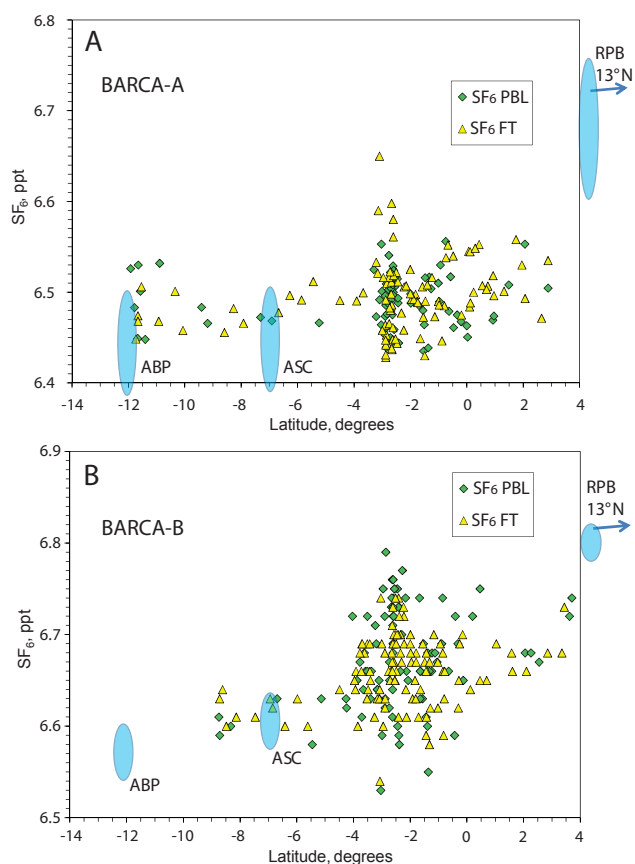
Fig. 3. Mixing ratios of sulfur hexafluoride ( SF_6 ) versus latitude, measured in flask samples taken during BARCA-A (A) and BARCA-B (B). The values obtained simultaneously at the NOAA monitoring sites Ragged Point, Barbados (RPB), Arembepe, Brazil (ABP), and Ascension Island (ASC) are indicated for reference.
