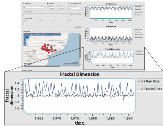
Figure 1: ClimFractal - D_2 measures.
