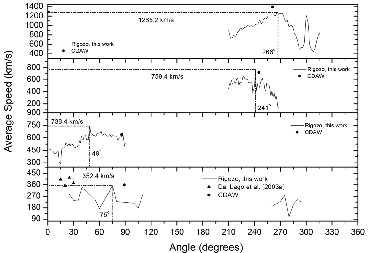
Figure 5 – Radial speed in function of the angle for the CME events on the following days: (A) September 28 (1997), (B) February 2 (2001), (C) March 1 (2002) and (D) December 2 (2003). It is possible to visualize the CME higher speed direction (shown with dotted lines).
