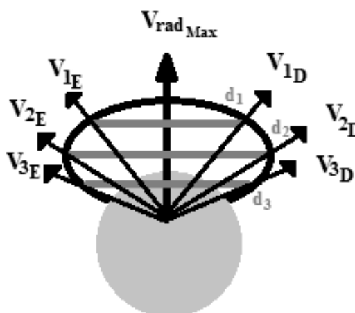
Figure 7 – Illustration of how the method determines the expansion speed ( V_{exp} ) of a CME event. Where V_{rad_{max}} is the vector of higher radial speed, V_{1D} , V_{2D} , V_{3D} and V_{1E} , V_{2E} , V_{3E} are the pairs of speed vectors (to the left and right of V_{rad_{max}} ) and d_{1, 2, 3} represent the distances between their respective pairs of speed vectors.
