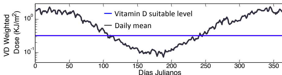
FIGURE 3. Annual variation of daily average dose of Vitamin D.
