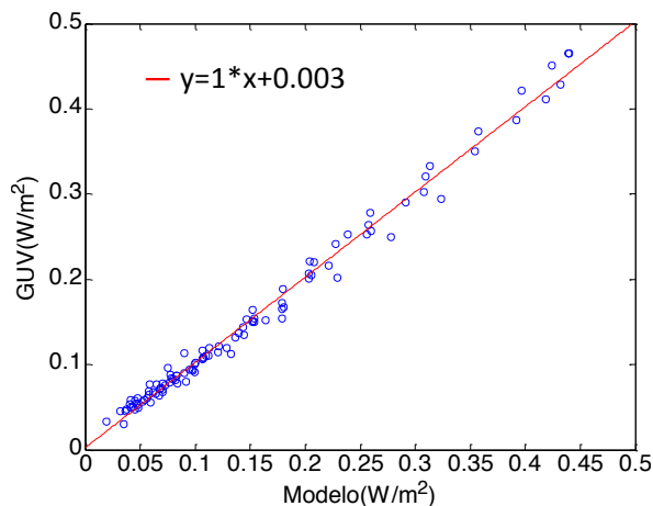
FIGURE 1. Correlation of UV_{vitD} obtained by GUV and modeled in clear sky conditions.
