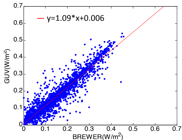
FIGURE 2. Validation. GUV and Brewer spectrophotometer correlation of UV_{vitD} in all sky conditions between October 2008 and December 2009.
