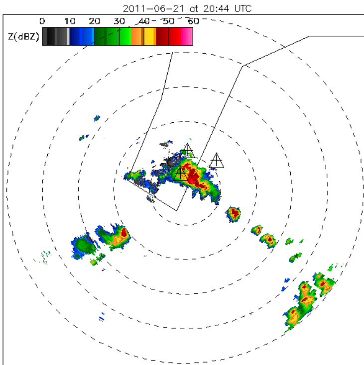
Figure 2. MAXCAPPI at 20:40
