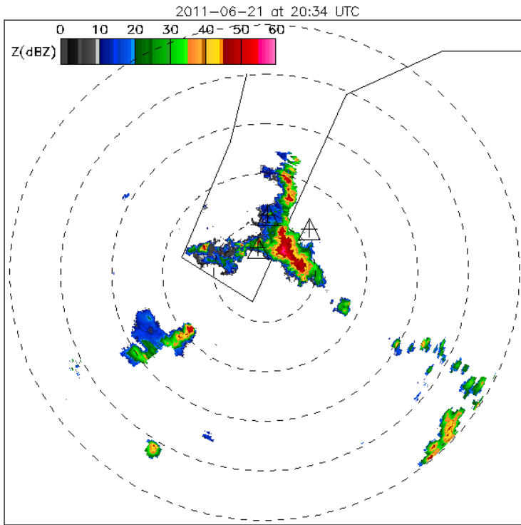
Figure 1. Position of field mill network and the radar image (MAXCAPPI) at 20:34.
