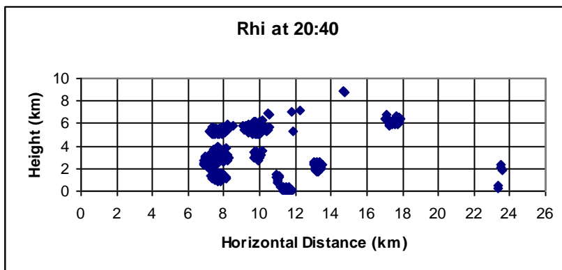
Figure 3. RHI (over Outeiro site) at 20:40. The regions in blue correspond to reflectivity more than 45 dBz.
