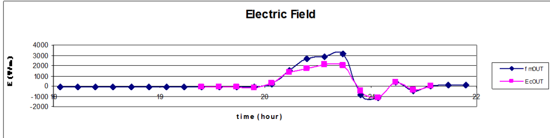
Figure5. Adjust of E_i \times E_{ci} during a thunderstorm at Outeiro position.
