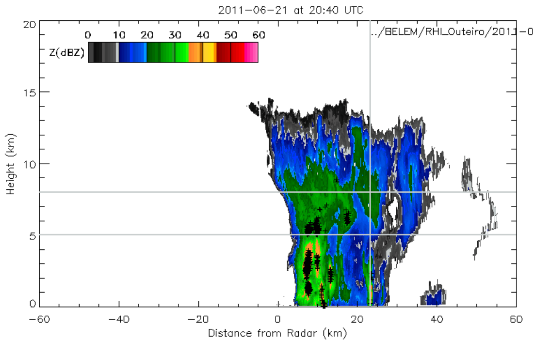
Figure 4. Representation of RHI during a thunderstorm. The black crosses represent regions with reflectivity greater than 45 dBZ. This figure was used to obtain figure 3.
