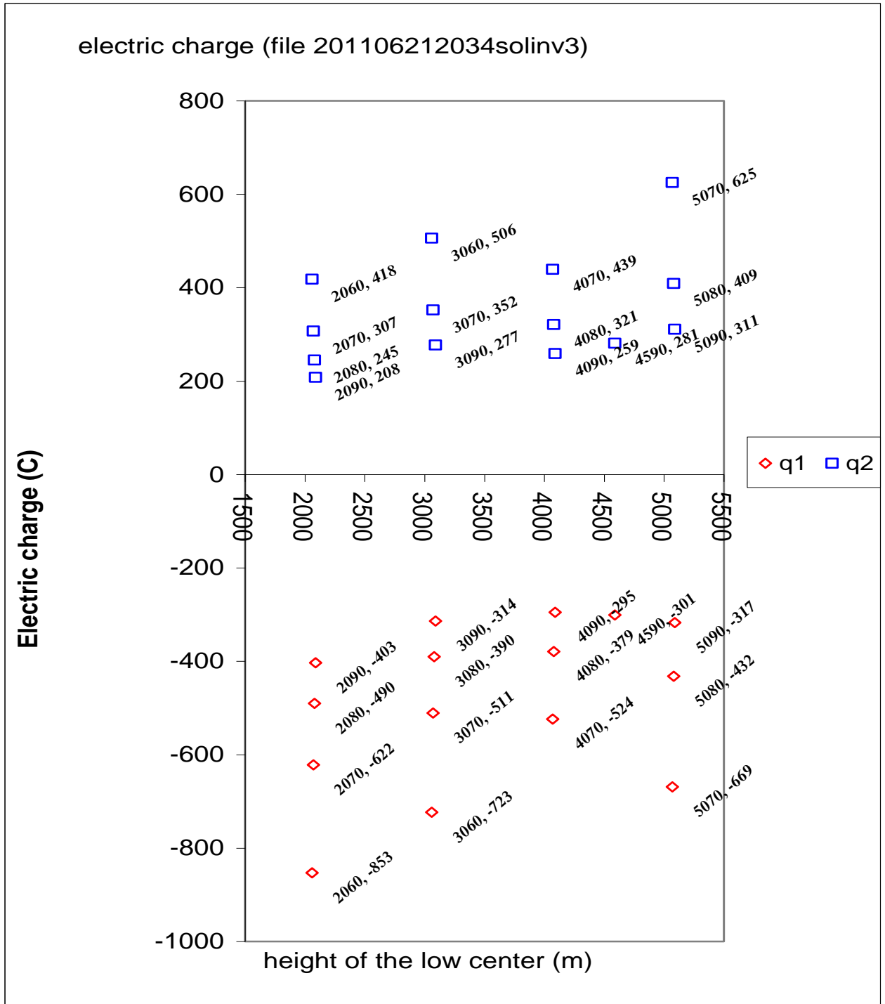
Figure 6. Solutions obtained for several positions of charge centers, using a dipolar structure. One solution is two points one square (blue) and a diamond (red) with the same label (for example 2060). The number after is the magnitude of charge.
