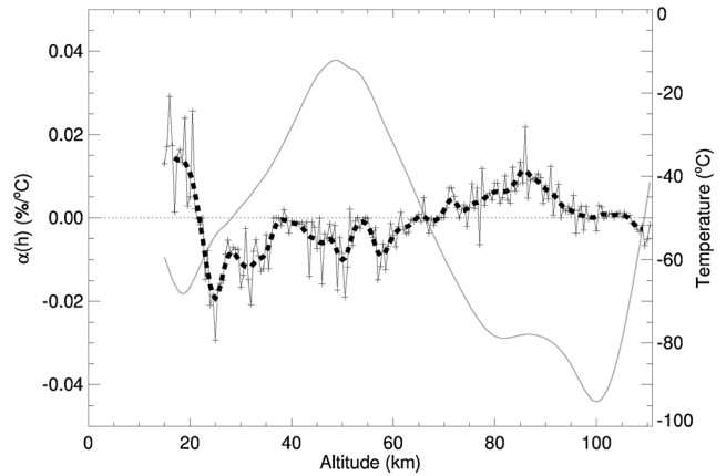
Figure 7. The continuous curve with crosses represents \alpha(h) values obtained. The black dashed curve represents the smoothing of these values and the continuous grey curve represents the typical temperature altitude profile observed by the SABER instrument.
