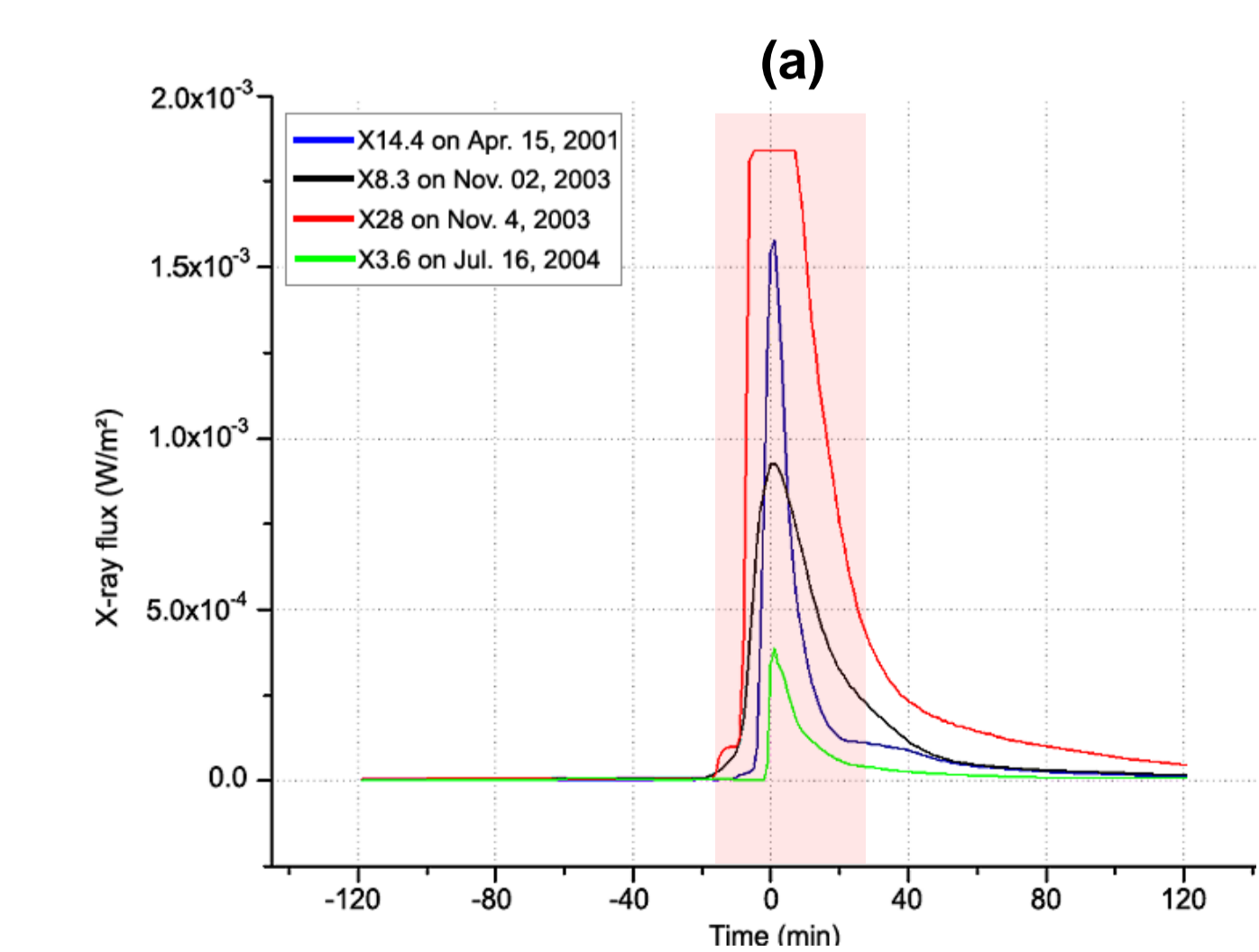
(a) The four selected flares in X-ray flux (0.1-0.8nm) and (b) the EUV count rate in 26.0–34.0nm. The full disc solar background has been removed from each event.
