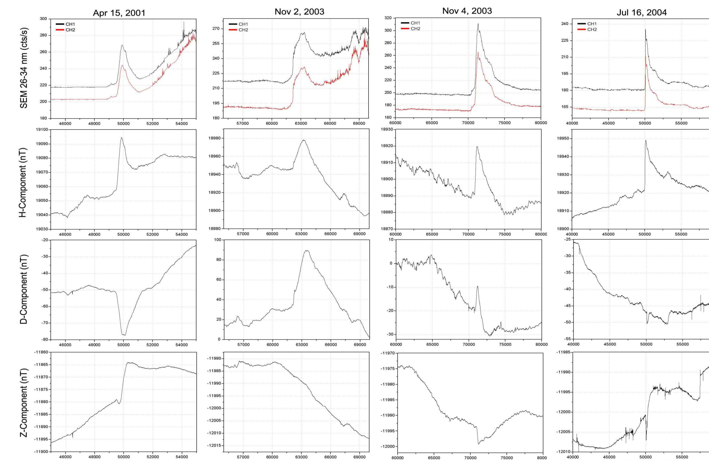
The EUV count rate and the variation of the geomagnetic field components (H, D, Z) during events of the selected flares.
