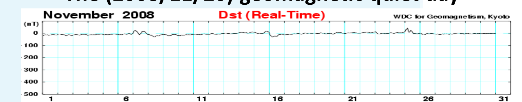
Figure 6 - DST Index, November 2008. Source: http://magdas.serck.kyushu-u.ac.jp/
