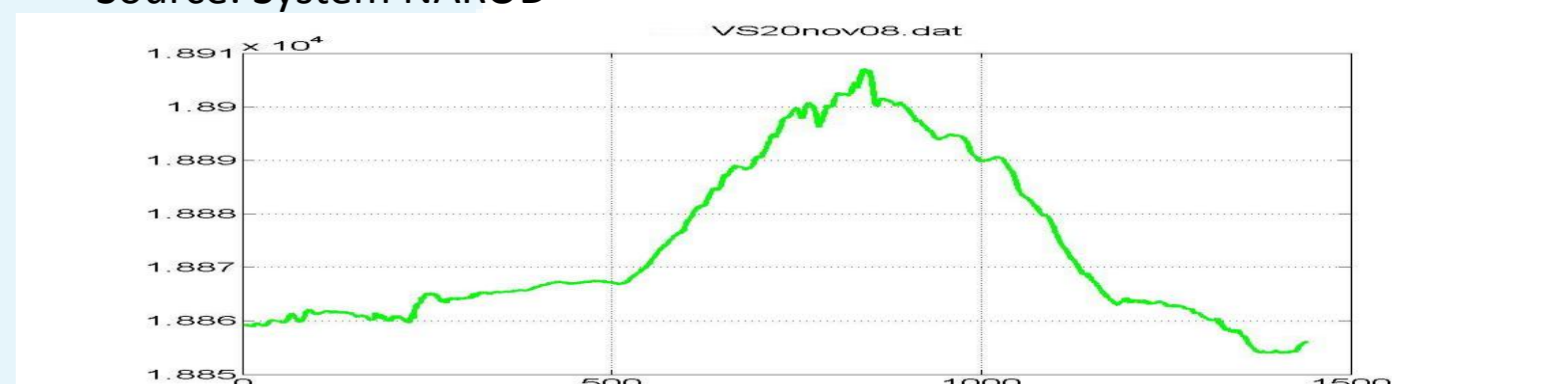
Figure 14 - Variation of the H component of geomagnetic field observed in the VSS/ON- MCT for 2008/11/20. Source: System NAROD
