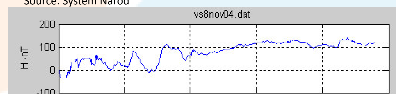
Figure 13 - Variation of the H component of geomagnetic field observed at the VSS/ON- MCT for 2004/11/08. Source: System NAROD
