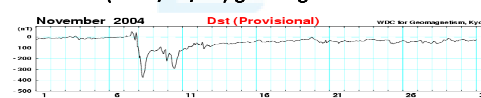
Figure 5 – DST Index, November 2004. Source: http://magdas.serck.kyushu-u.ac.jp/
