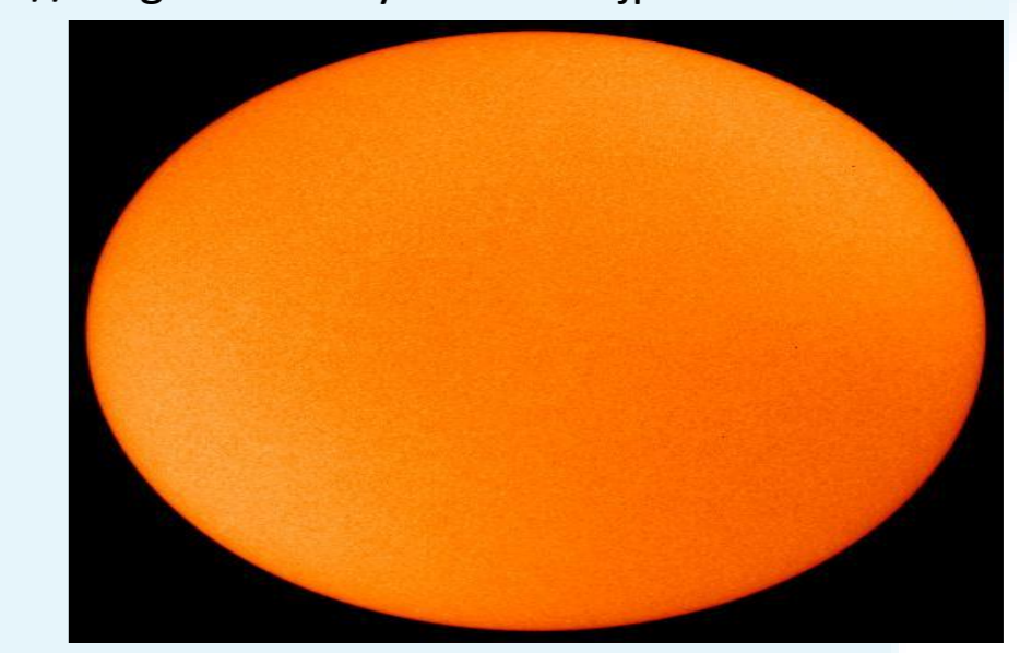
Figure 8 - No sunspots 2008/11/20. Source: SOHO / MDI
