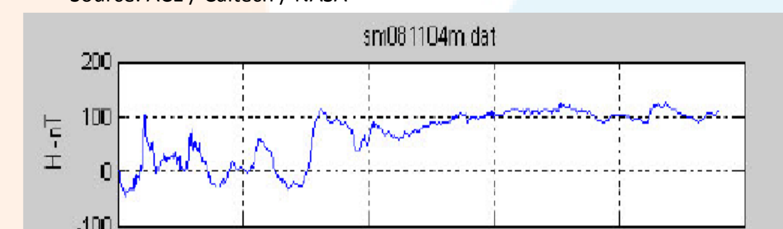
Figure 11 - Variation of the H component of geomagnetic field observed at the SSO/CRS/CCR/INPE–MCT for 2004/11/08. Source: System NAROD
