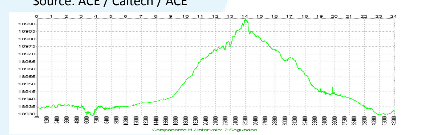
Figure 12 - Variation of the H component of geomagnetic field observed at the SSO/CRS/CCR/INPE–MCT for 2008/11/20. Source: System NAROD
