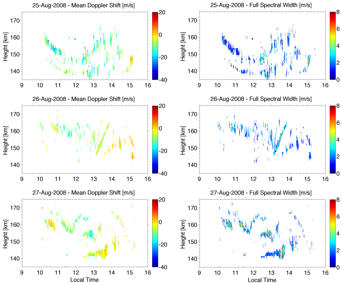
Fig. 4. Mean Doppler velocities (left-side panels) and full spectral widths (right-side panels) for \text{SNR} > -5 dB echoes observed on 25, 26 and 27 August 2008.
