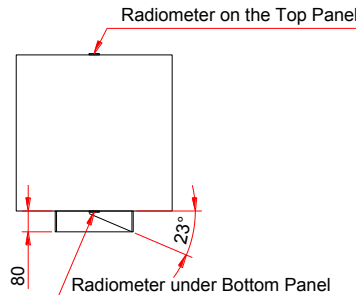
Figure 9. Proposed Positioning of the radiometers.
