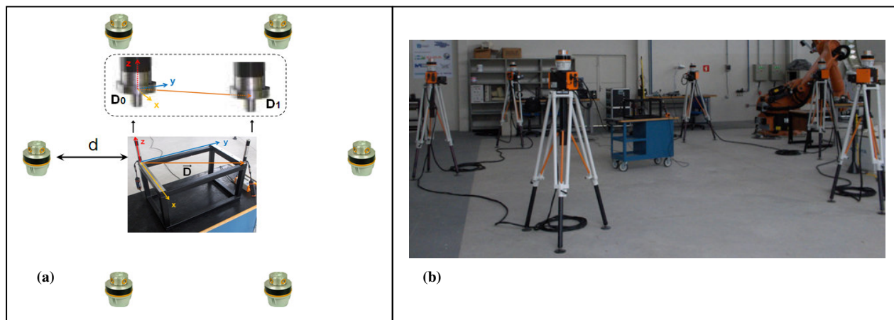
Figure 3. Experimental configuration: (a) Transmitter and sensors layout position around the sample test. (b) Transmitters position around sensors located on the sample test. Source: Landeta and Sutério (2010)
