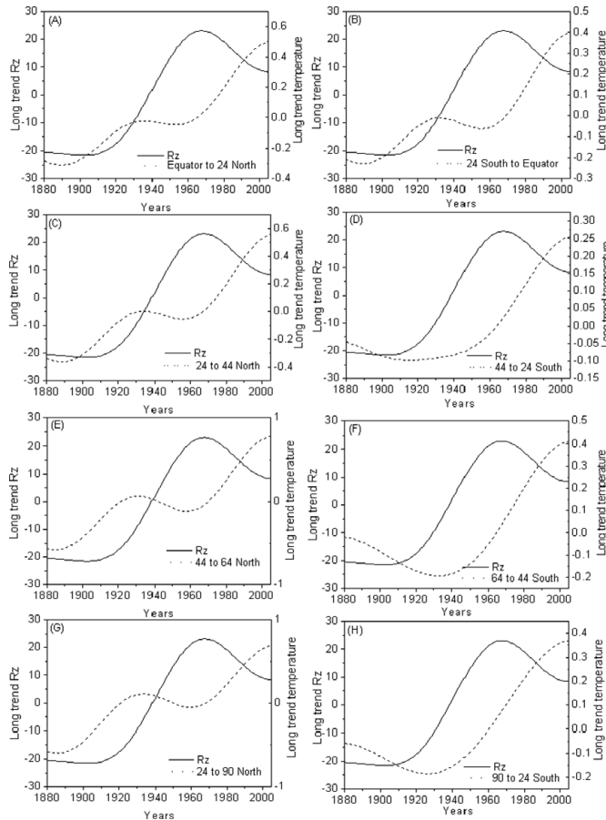
Figure 2. Long term trend for sunspot number (solid line) and for surface temperature (dotted lines). Panels show, on the left, latitudinal trends temperature long term trend for (A) 00^{\circ} - 24^{\circ} N, (C) 24 - 44^{\circ} N, (E) 44 - 64^{\circ} N and (G) 24 - 90^{\circ} N averaged temperatures; on the right, temperature long term trend for (B) 00^{\circ} - 24^{\circ} S, (D) 24^{\circ} - 44^{\circ} S, (F) 44 - 64^{\circ} S and (H) 24 - 90^{\circ} S averaged temperatures
