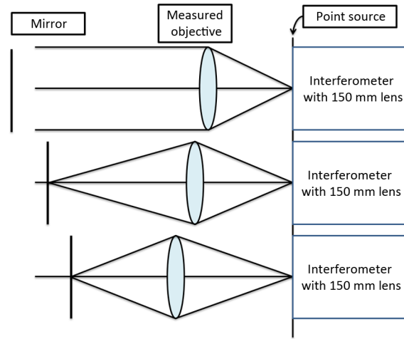
Fig. 5 The way to find the conjugates for focal length calculation using the interferometer and a mirror.
