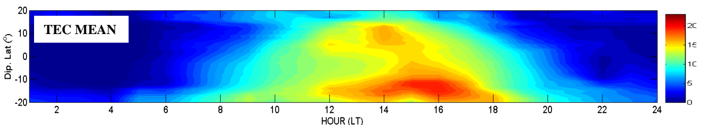
Figure 3: 10 days mean of TEC (TECU) from 3 - 12 Jan 2009 along the geomagnetic meridian of 60°W
