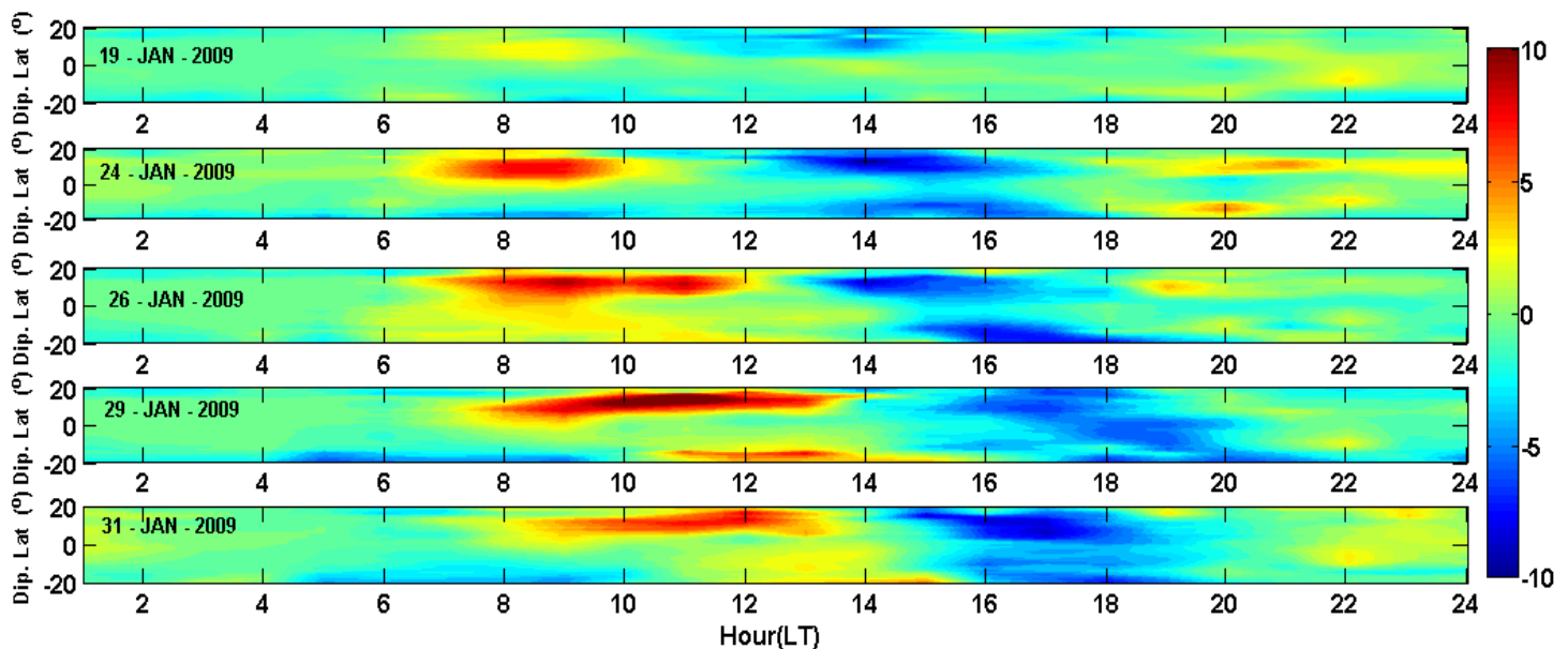
Figure 4: Change in TEC (TECU) during the SSW event of 2009 along the geomagnetic meridian of 60°W
