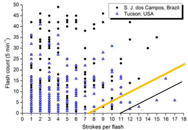
Figure 7 – Scatterplot of the flash count and flash multiplicities observed by high-speed cameras in São José dos Campos (black circles) and Tucson (blue triangles).
